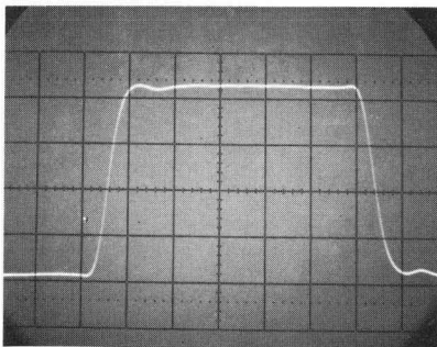
Fig. 6. Oscilloscope of typical pulse response of -hp-1110A probe operating directly into high-impedance oscilloscope ( -hp-175A/1751A ).
