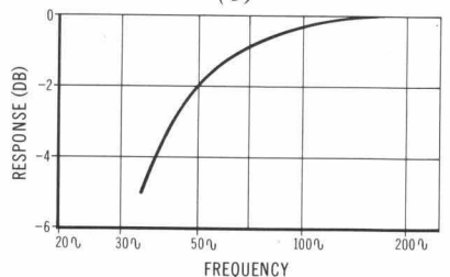
TYPICAL LOW-FREQUENCY RESPONSE OF -hp- MODEL 1110A PROBE WITH 1111A AMPLIFIER (d)
