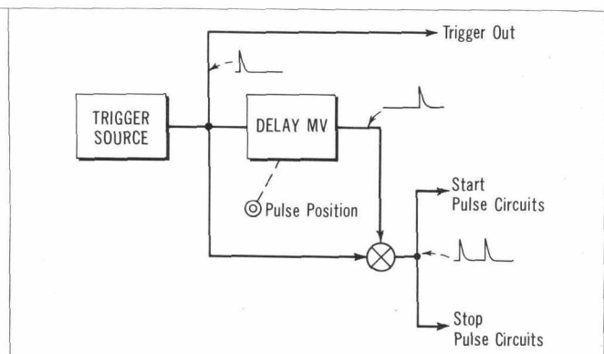
Fig. 8. Double pulse configuration uses Pulse position delay multivibrator to trigger main pulse circuits for second time.
