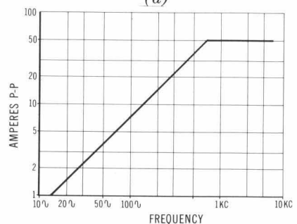
MAXIMUM CURRENT RATING OF -hp- MODEL 1110A PROBE WITH 1111A AMPLIFIER (f)
