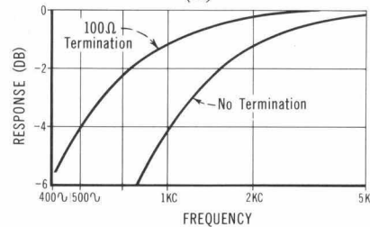
TYPICAL LOW-FREQUENCY RESPONSE OF -hp- MODEL 1110A PROBE (c)
