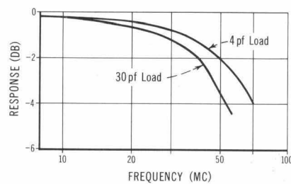
TYPICAL HIGH-FREQUENCY RESPONSE OF -hp- MODEL 1110A PROBE WITH 100-OHM TERMINATION (-hp- 10100B) (a)
