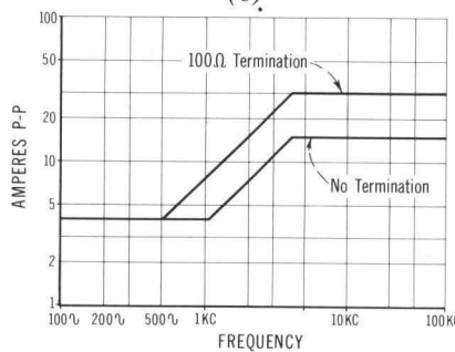
MAXIMUM CURRENT RATING OF -hp- MODEL 1110A PROBE (e)
