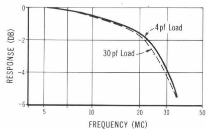
TYPICAL HIGH-FREQUENCY RESPONSE OF -hp- MODEL 1110A PROBE WITH 1111A AMPLIFIER USING 3' OF 50-OHM CABLE (b)
